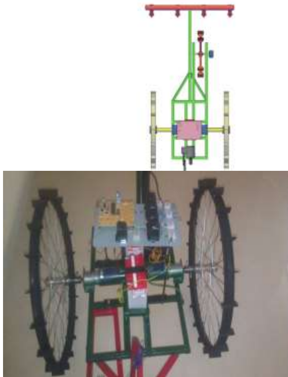
FIGURE3. Differential Drive steering axle
