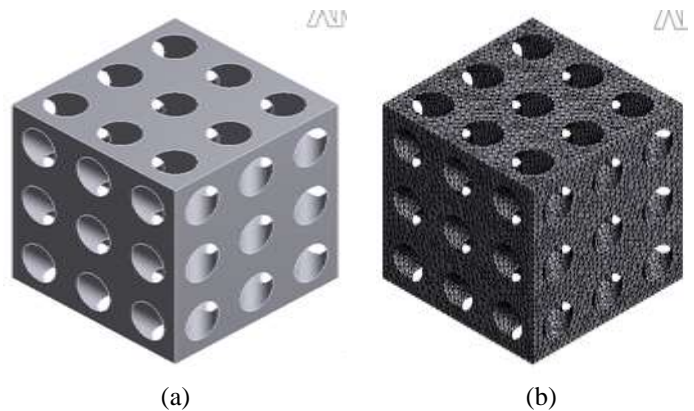
Figure 3. 3x3x3 Matrix of the single cell to produce 3D cubic porous solid model (a), mesh of the cube matrix (b)
