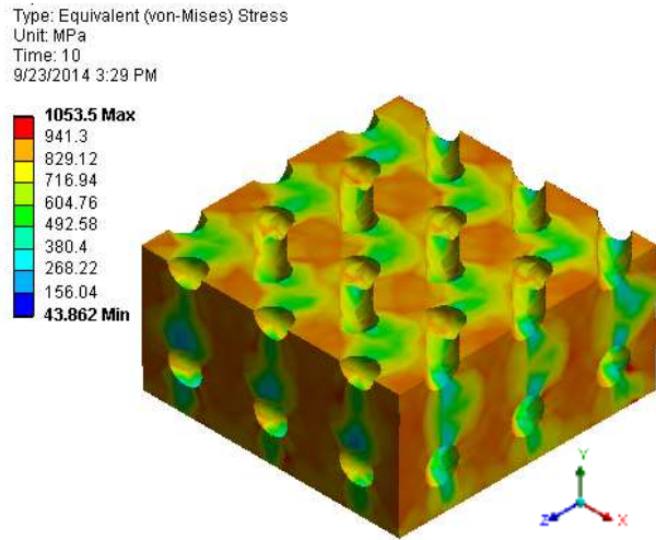
Figure 6. Equivalent Stress distribution of hole radius of 0.4 mm with cross section on y axis.
