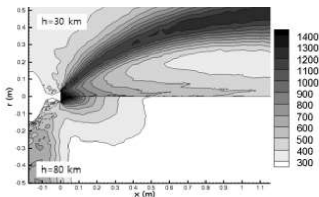
Figure. 9 Temperature contour of plume at h=30 km and 80 km.
