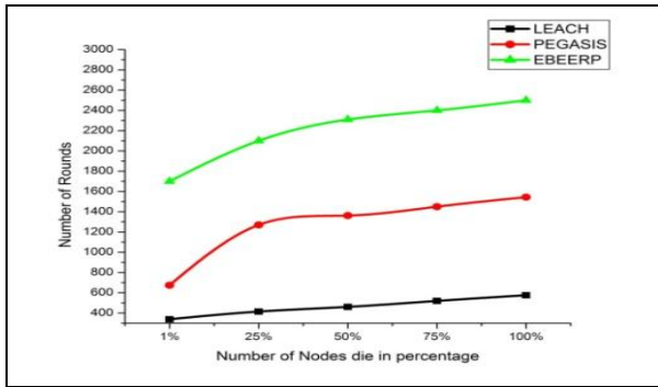
Figure 4: Experimental result for 100m X 100m network with initial energy 0.5 J/node
